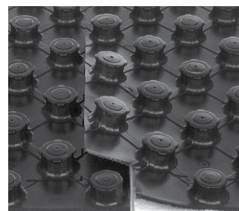
Overlap the edges of the Nexxa Panels.
